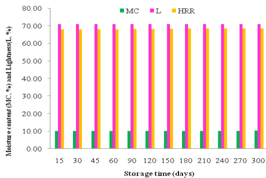
Fig. 4: Effect of moisture content on L and HRR of paddy stored in super grain bag
