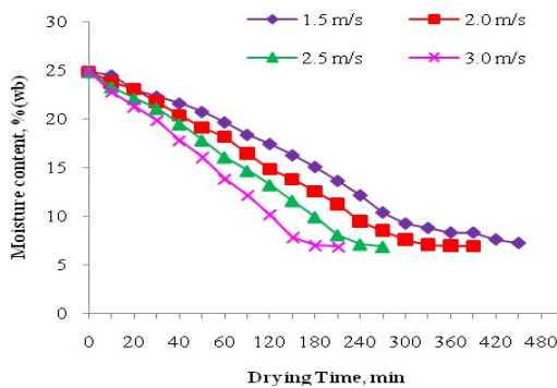
Fig. 3: Effect of air velocity on drying curve at different air velocity
